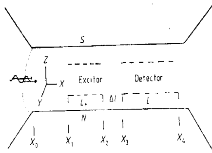
Fig. 1: Diagram of the model CW NMR Excitation Scheme with Separate Movable Detection System for accurate estimation of V_0 , V_{\text{pulse}}^0 and also the total cross-section of the blood vessel. L_e is the length of the excitor coil and \Delta L is the separation of the excitor and the detector coil whose length is L .
