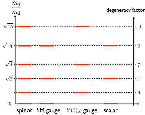
FIG. 2: Tree level KK mass spectrum for the spinor, SM gauge, U(1)_X gauge, and scalar fields. The mass splitting due to the electroweak symmetry breaking is neglected.
