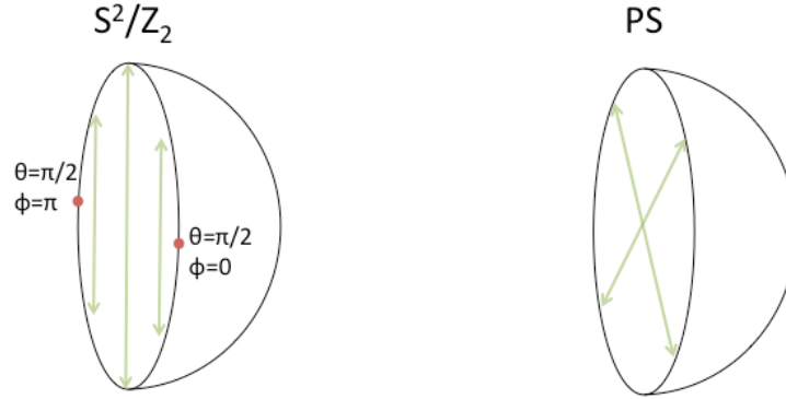
FIG. 1: S^2/Z_2 orbifold and PS manifold for left and right panels, respectively, when we take the fundamental domain as 0 \leq \phi \leq \pi . Arrows denote the identification on the boundary. Dots on the left panel indicate the orbifold fixed points.
